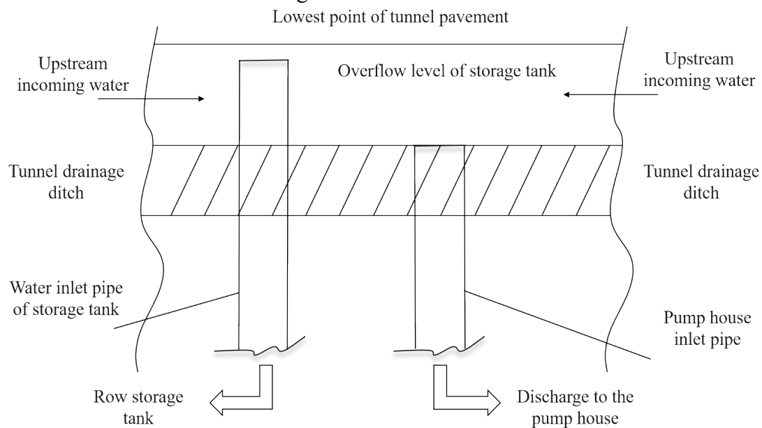
Figure 1 Design of rainwater runoff diversion facilities
